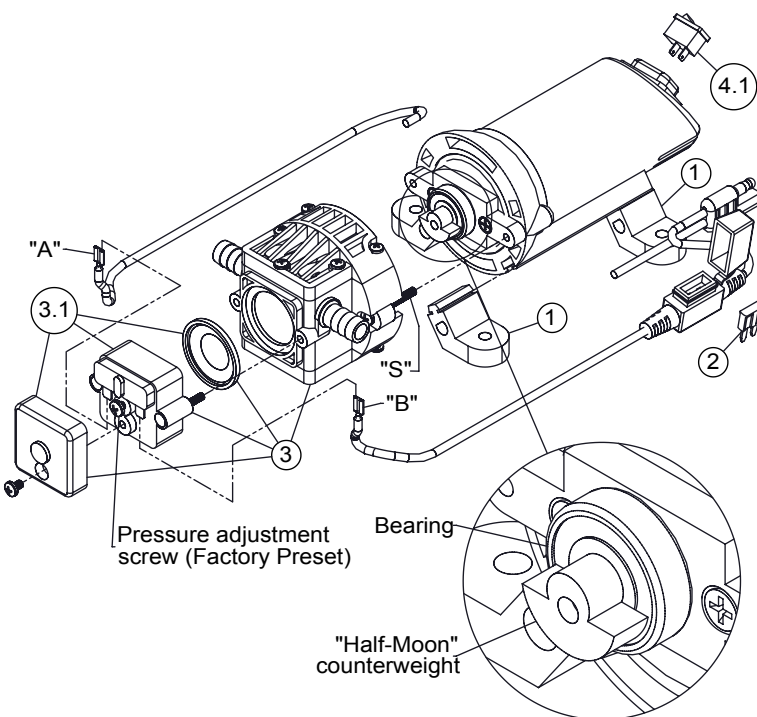
#5275702 Pump (12 Volt, 4 Amp, 1.0 gpm, 35 psi)
